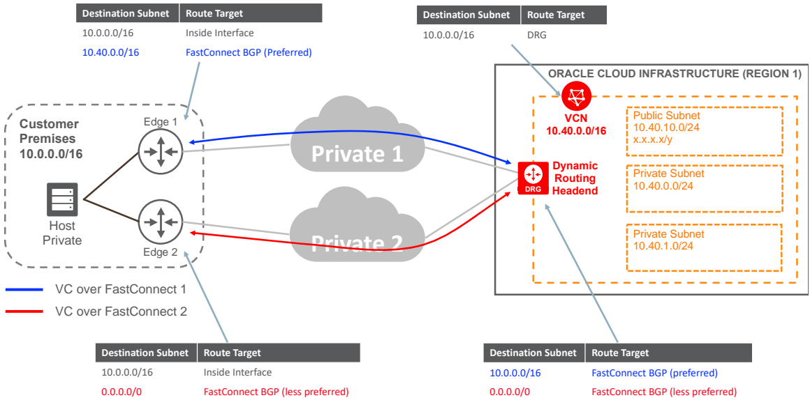
Figure 11. Redundant FastConnect—Routing
