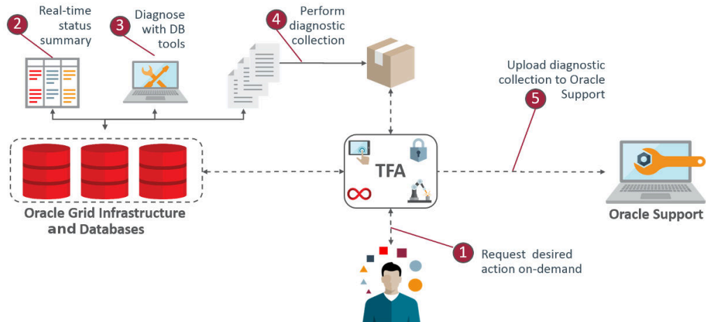
Figure 14-1 On-Demand Collections
