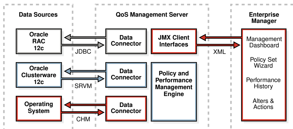
Figure 6-6 Diagram of Oracle Database QoS Management Server Architecture
