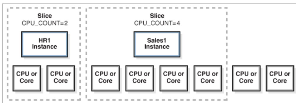
Figure 6-1 Instance Caging and CPU Slices
