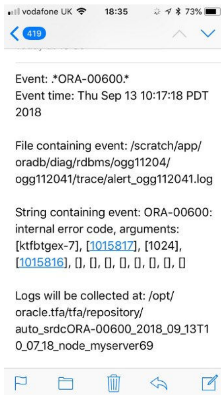
Figure 16-1 Email Notification
