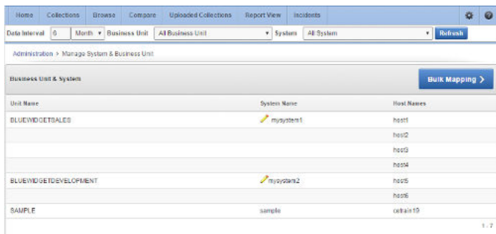
Figure 2-12 Bulk Mapping
