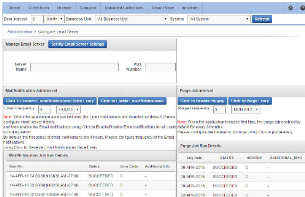
Figure 2-15 Configure Purging
