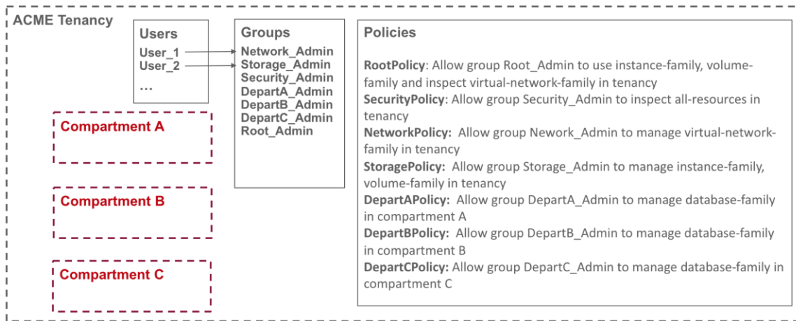
Figure 3. Scenario for Compartment and Policy Design
