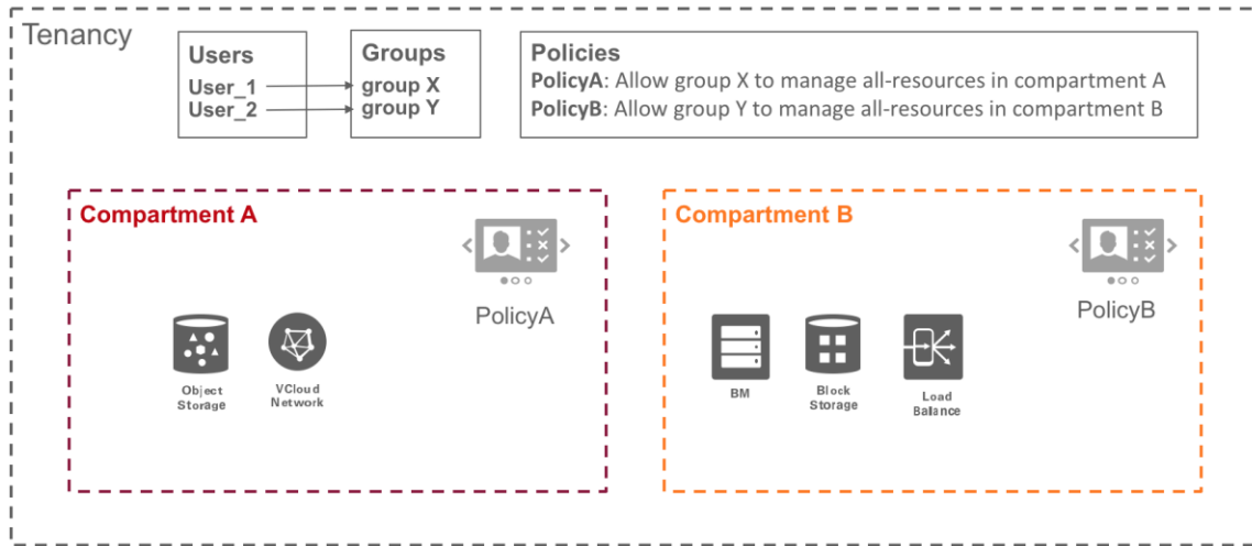
Figure 1. Oracle Cloud Infrastructure IAM Service Components
